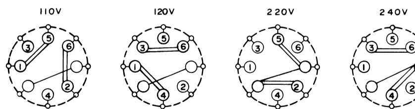
VOLTAGE SELECTOR CONNECTION
